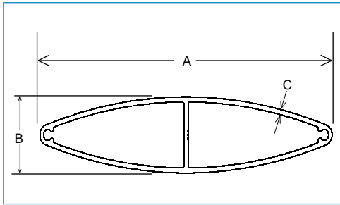
Elliptical Louvre
